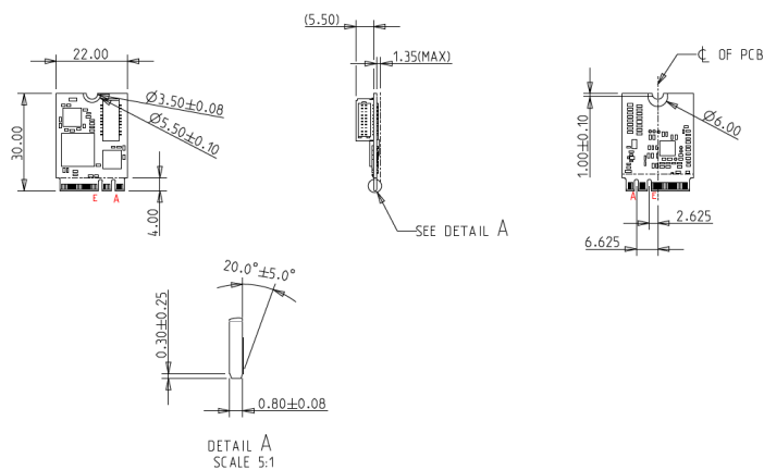
EGP2-X201-W2 (Horizontal Connector)
